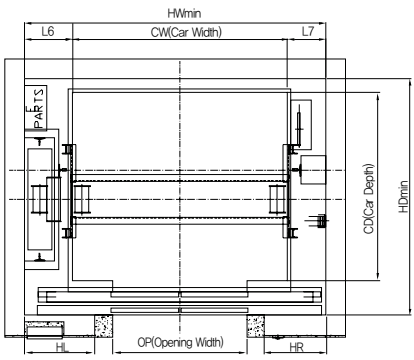
(Passenger / Simplex)
