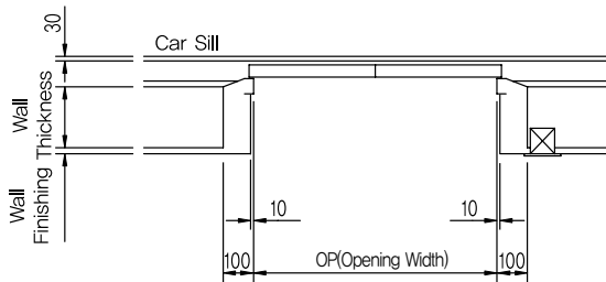
View B-B
