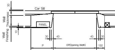
Wide Taper Type [ View B-B ]
