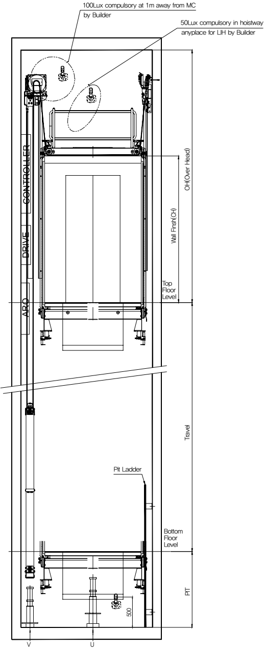
Hoistway Section
